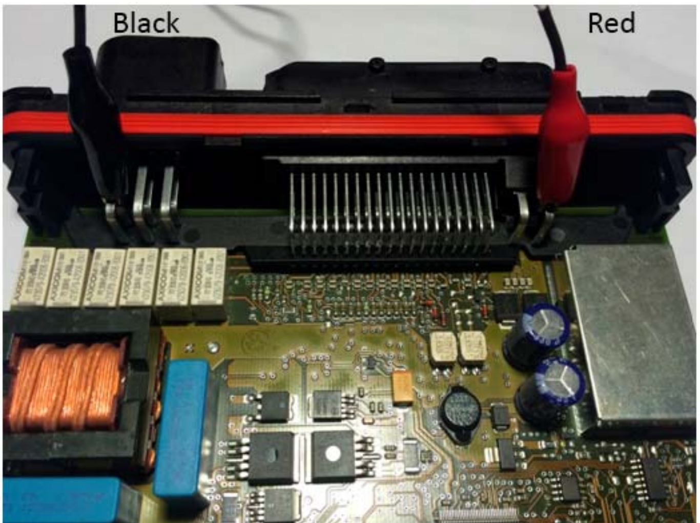
Pic.5 Crocodile - connectors cable plugging
